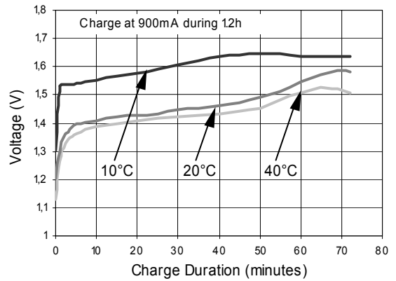
Fast Charge Characteristics
