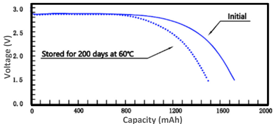
Aging Discharge Characteristics at +20 \pm 2 \text{ }^\circ\text{C}
