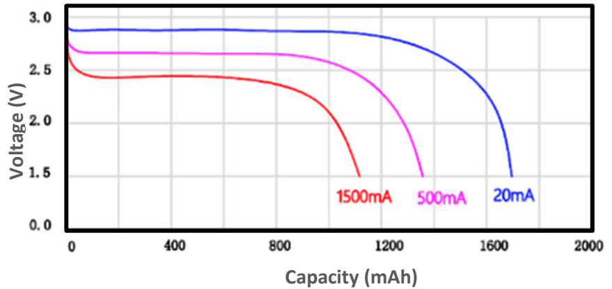
Typical Discharge Profiles at +20 \pm 2 \text{ }^\circ\text{C}
