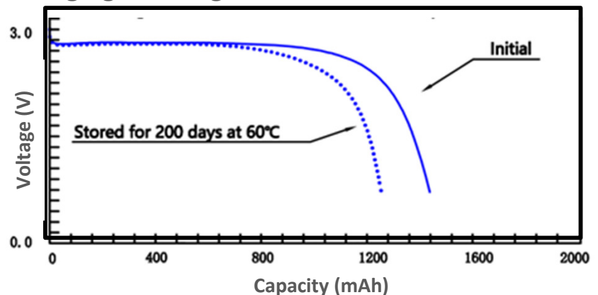
Aging Discharge Characteristics at +20 \pm 2 \text{ }^\circ\text{C}
