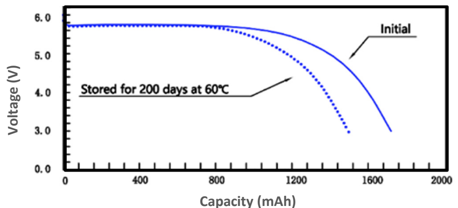
Aging Discharge Characteristics at +20 ± 2 °C
