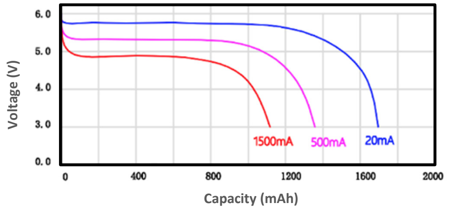
Typical Discharge Profiles at +20 ± 2 °C
