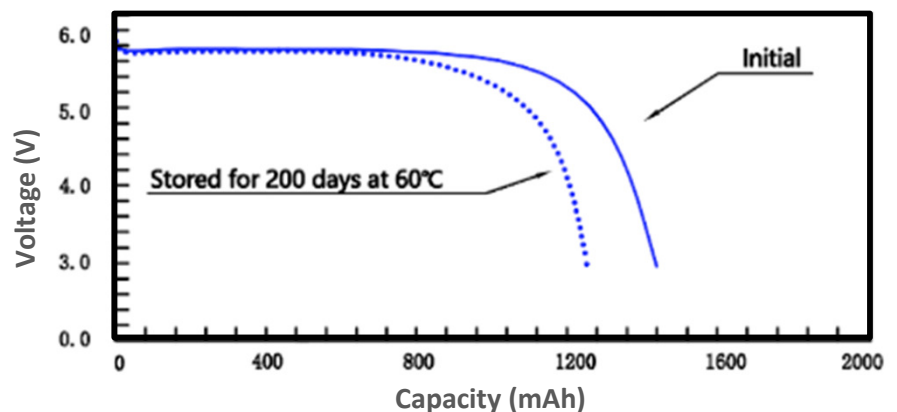
Aging Discharge Characteristics at +20 ± 2 °C
