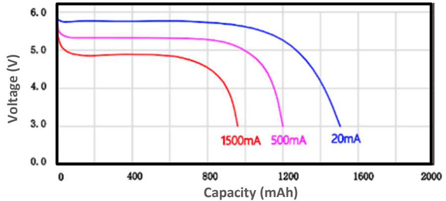
Typical Discharge Profiles at +20 ± 2 °C
